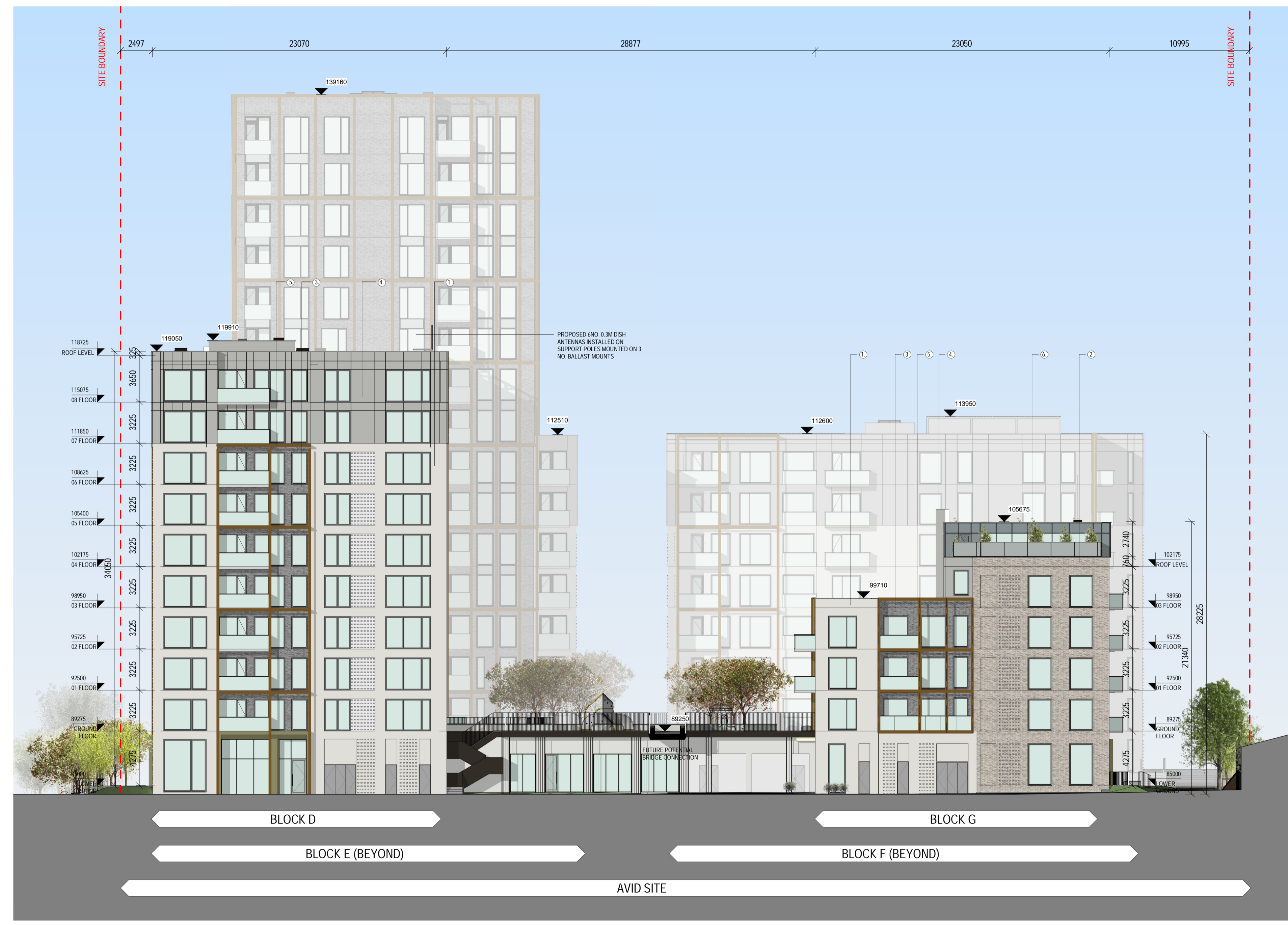
1 PROPOSED COURTYARD ELEVATION 02 - AVID SITE 1 : 200
